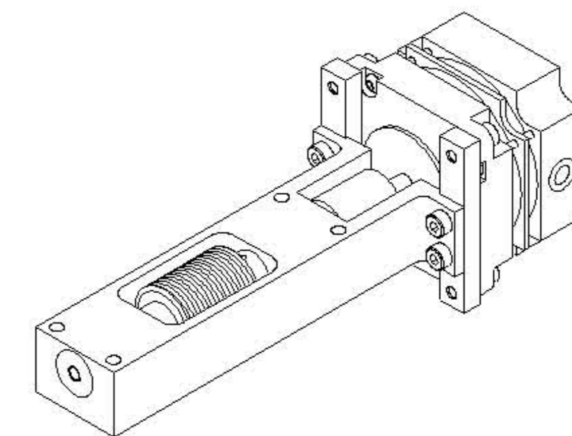
NOTcam motor and worm assembly
