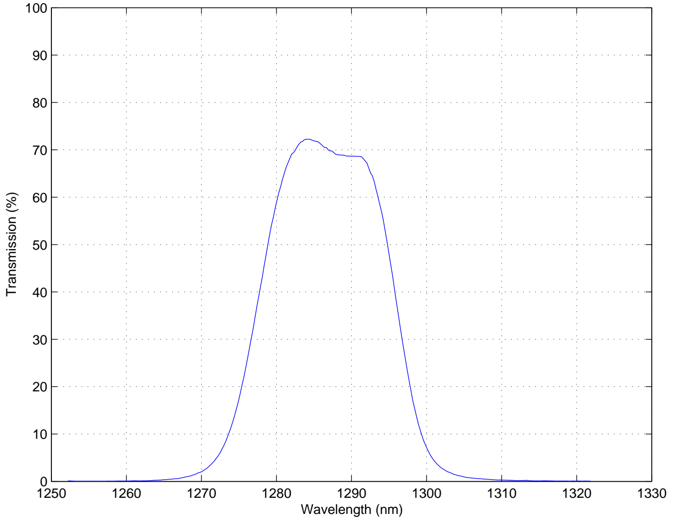
Filter #216, Pa-beta, vacuum wavelength, T=74K
