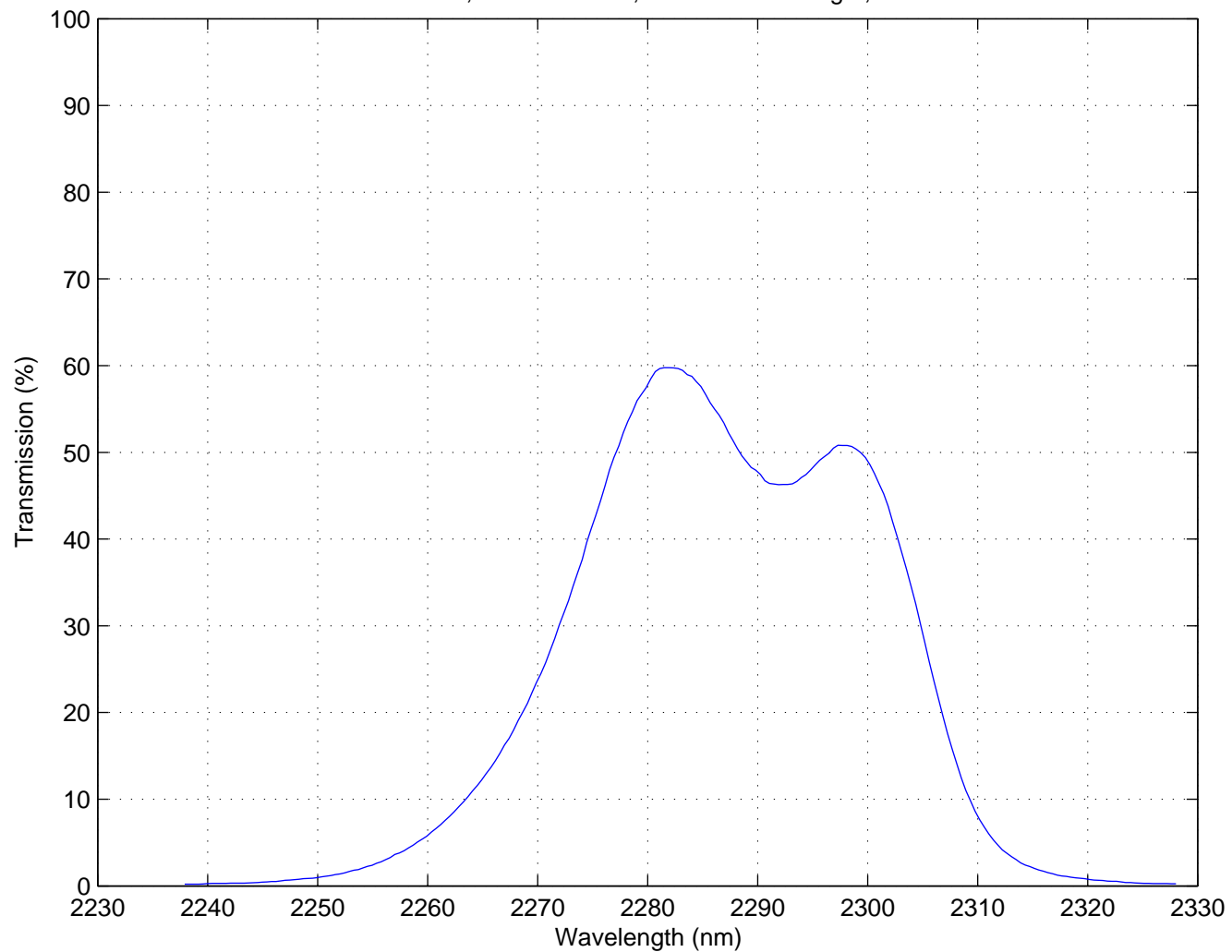
Filter #221, CO bandhead, vacuum wavelength, T=74K
